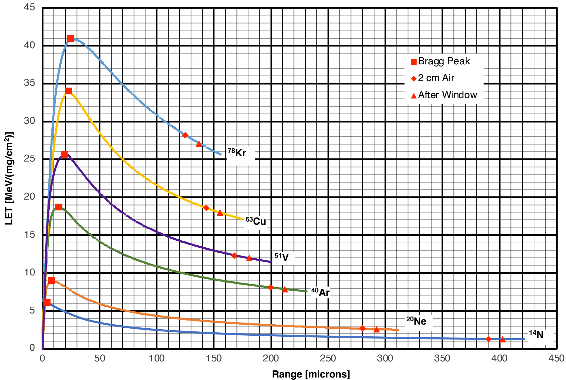
LET vs Range in Silicon for K150 15 MeV/u Beams
